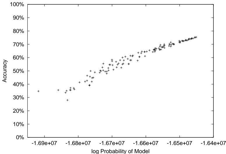
Figure 1.2 A scatterplot showing the correlation between the posterior model probability and the accuracy of a model trained with labeled and unlabeled data. The strong correlation implies that model probability is a good optimization criteria for the 20 News-groups dataset.
