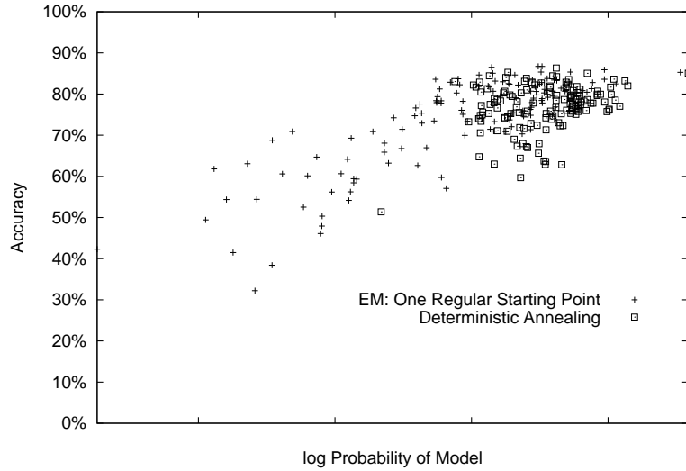
Figure 1.5 A scatterplot comparing the model probabilities and accuracies of EM and deterministic annealing. The results show that deterministic annealing succeeds because it finds models with significantly higher probability.
