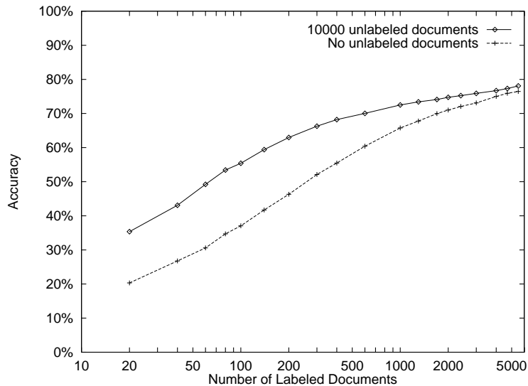
Figure 1.1 Classification accuracy on the 20 Newsgroups data set, both with and without 10,000 unlabeled documents. With small amounts of training data, using EM yields more accurate classifiers. With large amounts of labeled training data, accurate parameter estimates can be obtained without the use of unlabeled data, and classification accuracies of the two methods begin to converge.
