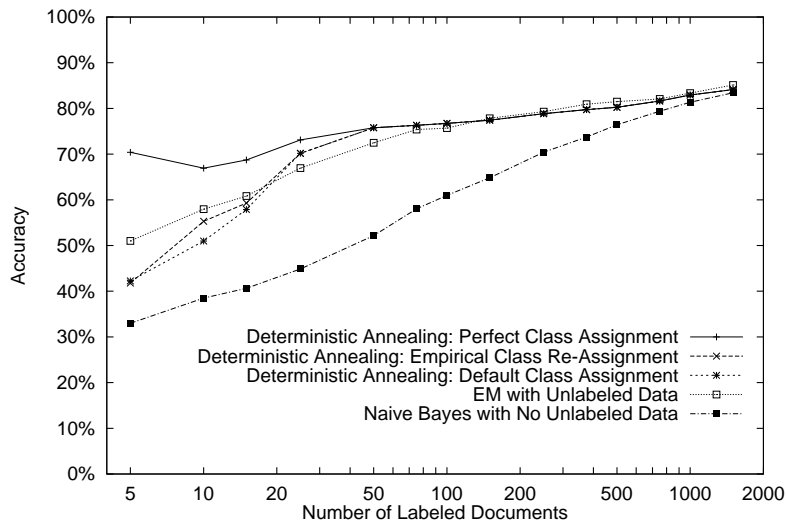
Figure 1.4 The performance of deterministic annealing compared to EM. If class-to-component assignment was done perfectly deterministic annealing would be considerably more accurate than EM when labeled data are sparse. Although the default correspondence is poor, this can be corrected with a small amount of domain knowledge.
