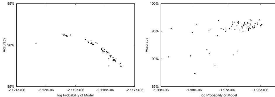
Figure 1.3 Scatterplots showing the relationship between model probability and classification accuracy for the Reuters acq task. On the left, with only one mixture component for the negative class, probability and accuracy are inversely proportional, exactly what we would not want. On the right, with ten mixture components for negative , there is a moderate positive correlation between model probability and classification accuracy.
